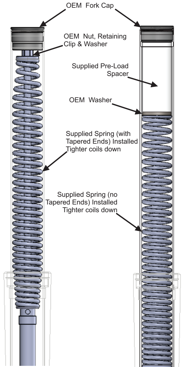
Left Fork with 110mm Fork Oil Level (5wt Fork Oil) See instructions to properly set oil level
