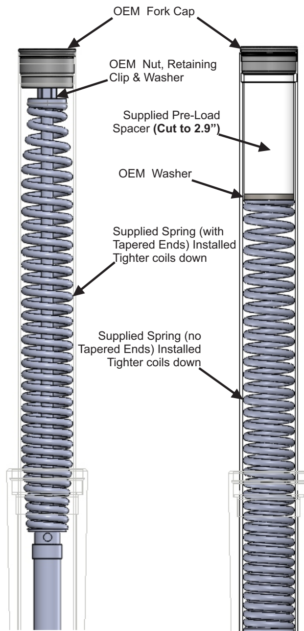
Left Fork with 110mm Fork Oil Level (5wt Fork Oil) See instructions to properly set oil level
